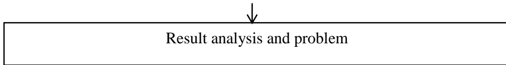
Figure 2.2: Flowchart
