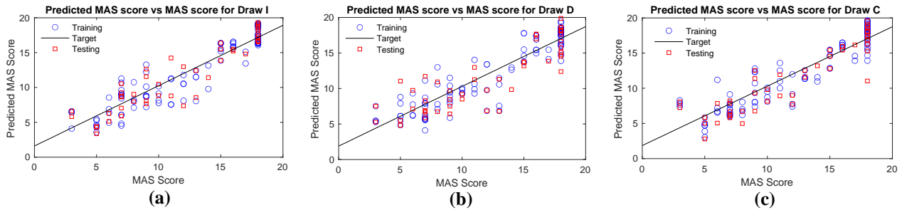
Fig. 2 - Predicted MAS score versus MAS score using ReHAD with feature selection of ( p < 0.05 ) of the kinematic variables for (a) Draw I module, (b) Draw D module and (c) Draw C module.
