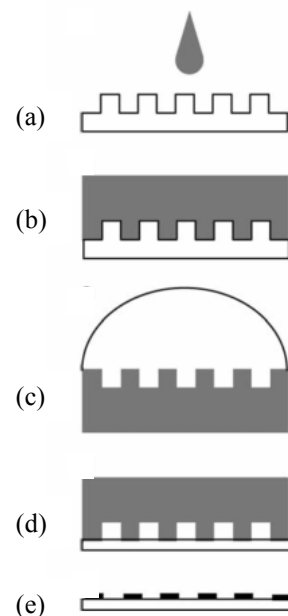
Fig.1. Schematics diagram of a \mu CP process. PDMS is applied to a master design (a) and allowed to cure (b), forming a mold/stamp. After peeling the stamp from the
