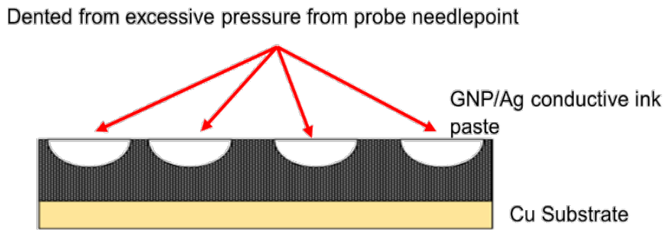
Fig. 11 Dented effect on conductive ink paste
