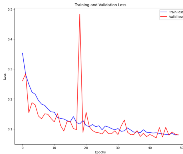
Fig. 5 Loss plot of the U-Net model modified with ResNet34
