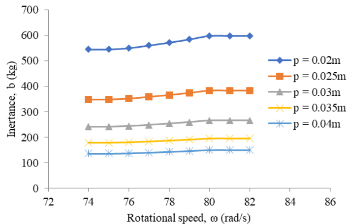
Fig. 6 - Comparisons between graph of inertaance against rotational speed of inerter flywheel with varying ball-screw pitch
