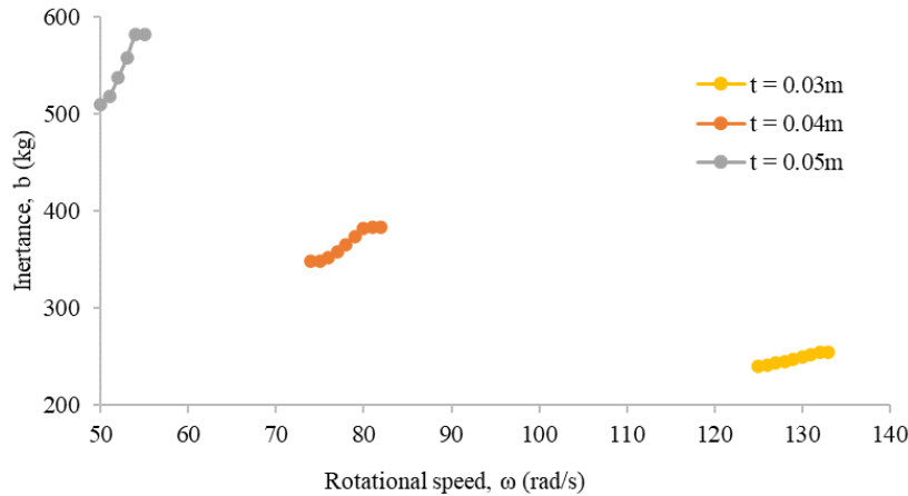
Fig. 5 - Comparisons between graph of inertaance against rotational speed of inerter flywheel with varying thickness (0.03m, 0.04m, 0.05m)
