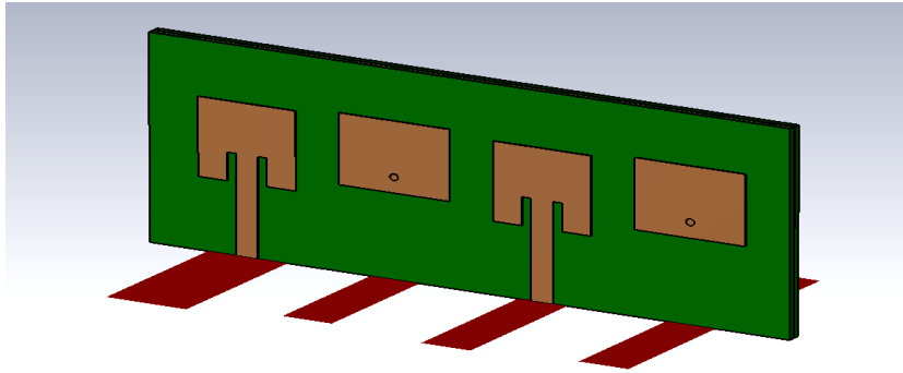
Fig. 12 - Rectangular patch antenna with via-hole patch antenna array with \lambda/2 spacing
