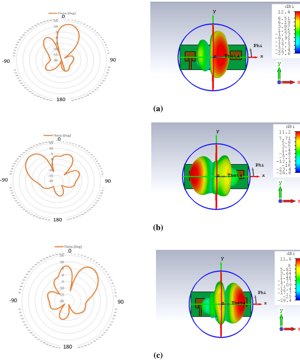
Fig. 12 - Rectangular patch antenna with via-hole patch antenna array with \lambda/2 spacing
