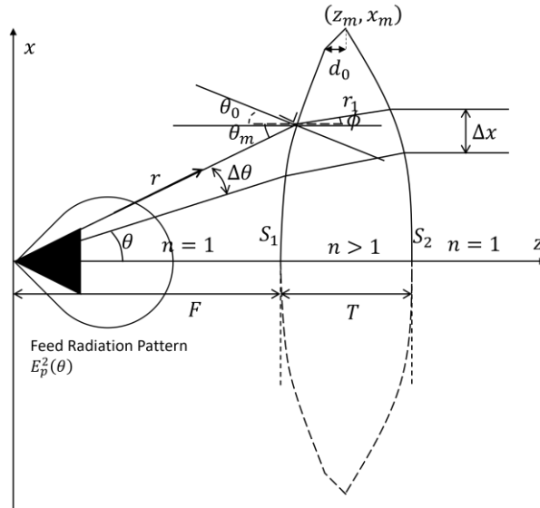
Fig. 3 - Concept of lens shaping
