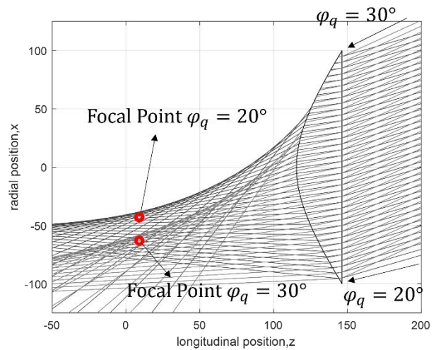
Fig. 8 - Results on hyperbolic planar lens (a) 0° and 10° incident angle; (b) 20° and 30° incident angle
