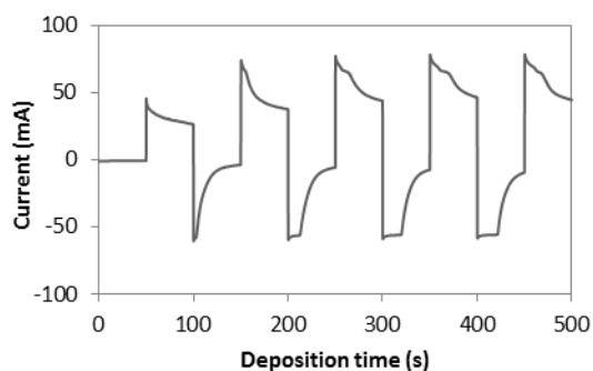
Fig. 1 The pulse-chronoamperometry curve for electrochemical reduction and deposition of rGO/MnO 2 composite using voltage of -1.0 V for 50 s and 1.0 V for 50 s per cycle with 0.2 M of Mn(Ac) 2 at the temperature of 40°C.
