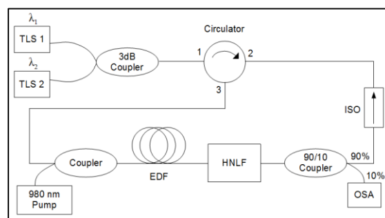
Figure 3 Schematic diagram for ring cavity multiwavelength fiber laser in experimental method.
